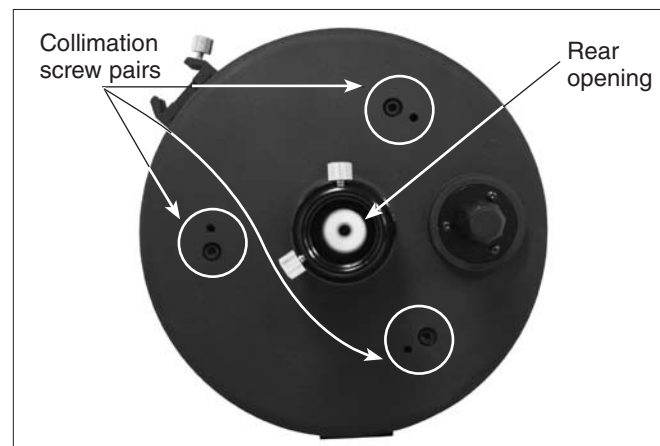
Figure 5. The 180mm Maksutov-Cassegrain screws
